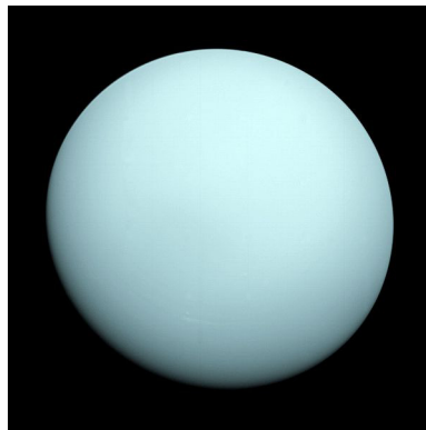
Uranus as seen by Voyager 2
